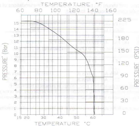
OPERATING PRESSURE TEMPERATURE 1/2" - 2" BALL VALVE
